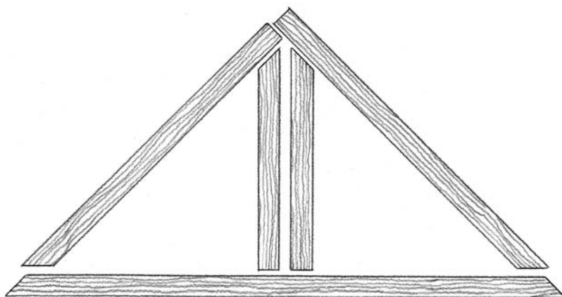
Figure 5-3: Sleeping shelf frame assembly.
