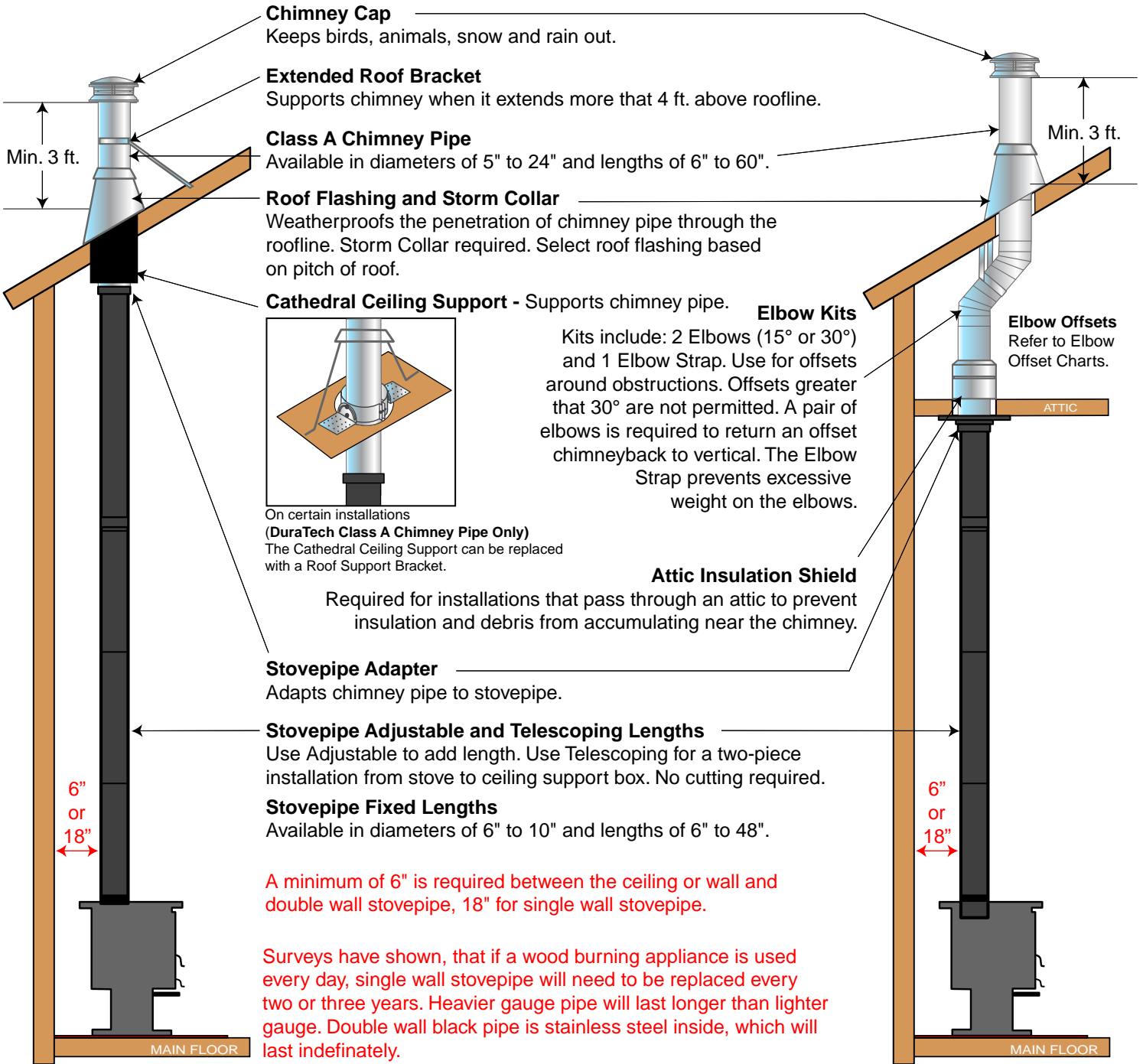
Cathedral Ceiling Support Installation
