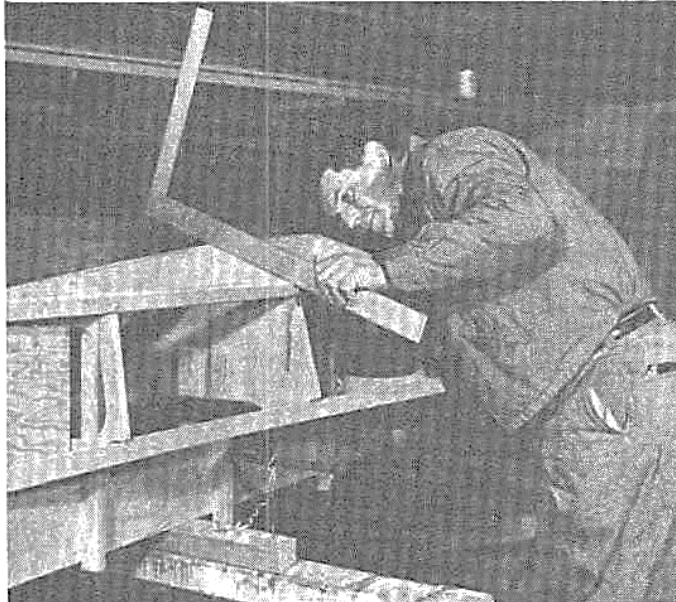
Fig. 2. Check as you go by holding straight edge against keelson, chine strip. Bevel on keelson, chine should conform to straight edge which should slide past frames, just touching.
