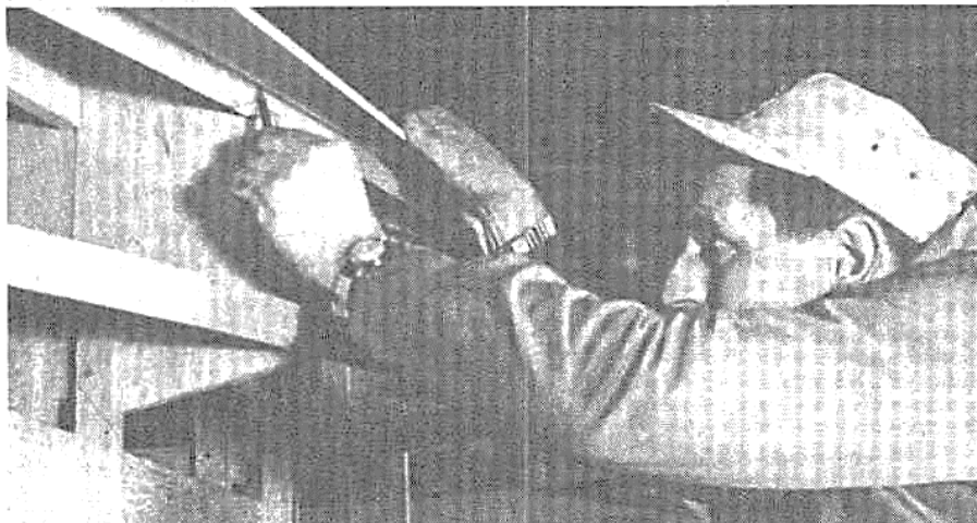
Fig. 3. Cut out bottom piece, leave extra material for trim. Because of curve in keelson, you'll have to trim edge of the planking to make it fit exactly.
