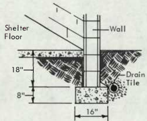
FOUNDATION DETAIL Family Shelter
