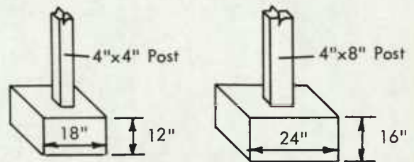
FOOTING DETAILS
