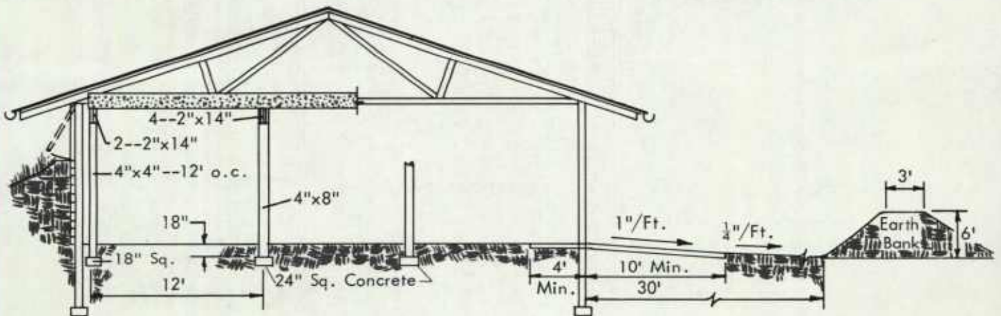
FOOTING DETAILS
