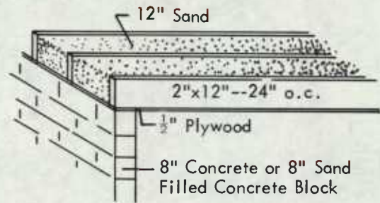
CEILING CONSTRUCTION Family Shelter
