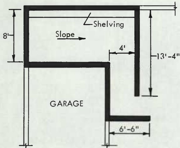
FLOOR PLAN
